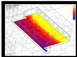
Daylight Analysis
